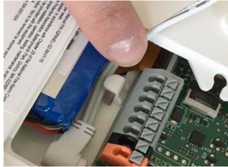
Route the wire behind the retainer clip
